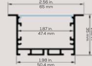
Recessed Direct
