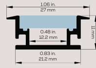
Recessed Accent
